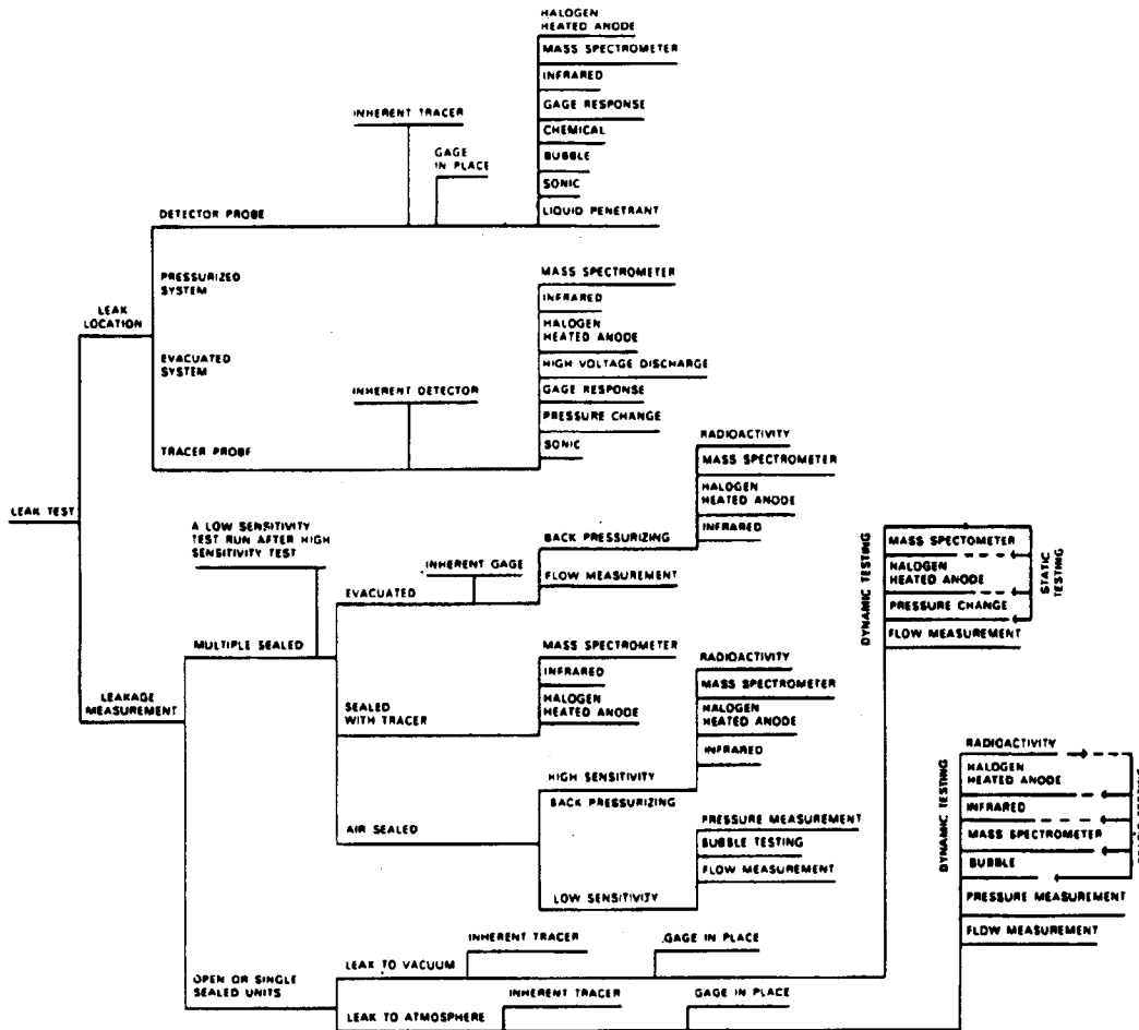
FIG. 1 Guide for Selection of Leakage Testing Method
