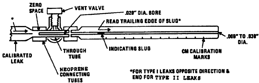
FIG. 3 Calibration Capillary and Vent Valve Assembly
