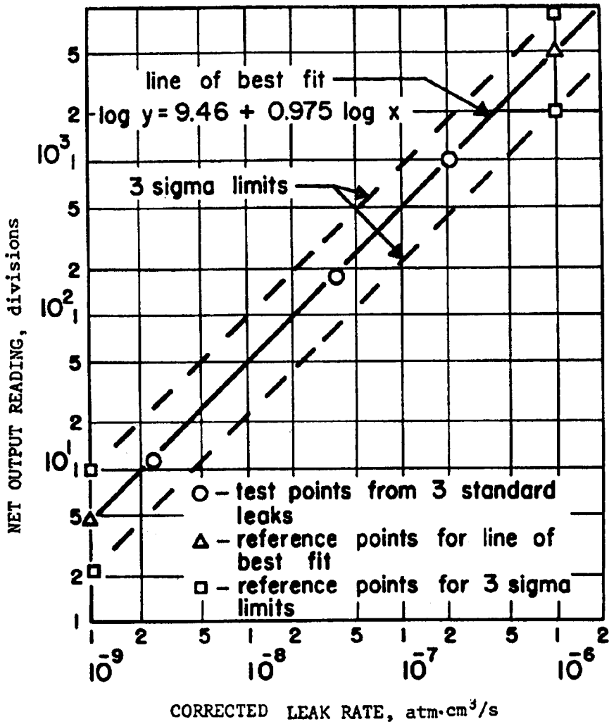
FIG. A1 Net Output Reading versus Corrected Leak Rate for Calibration of Helium Leak Detectors
